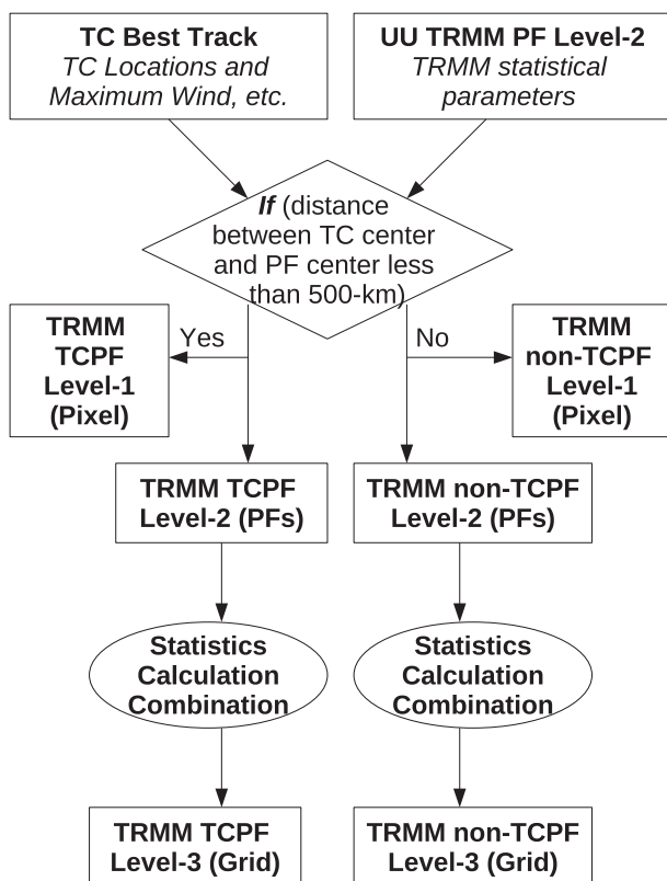
FIG. 1. FIU-UU TRMM TCPF database construction flowchart.
