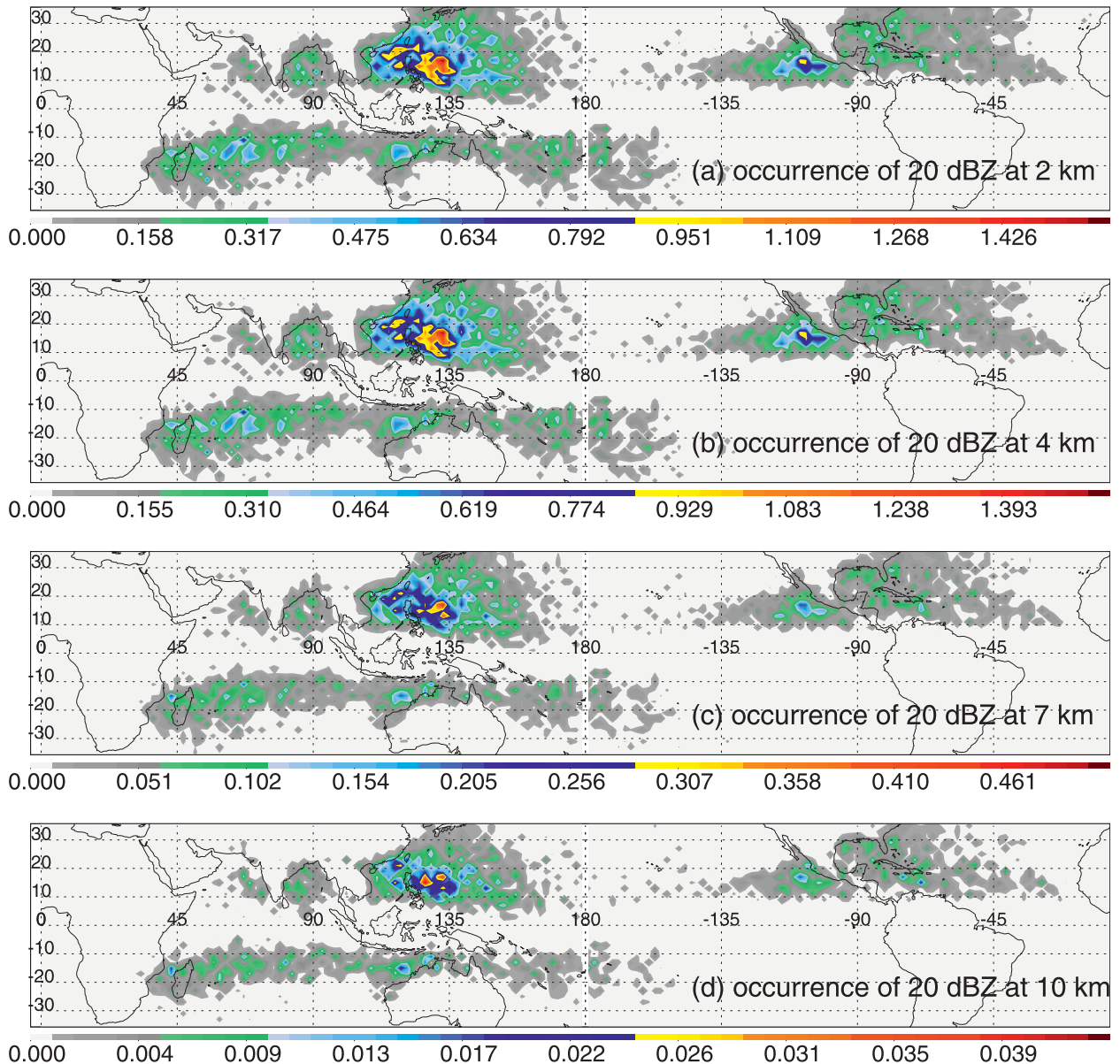
FIG. 10. Occurrence of PR reflectivity greater than 20 dBZ (%) at (a) 2, (b) 4, (c) 7, and (d) 10 km derived from TC RPPFs in 1998–2009. Note that the scales are different for (a)–(d).
