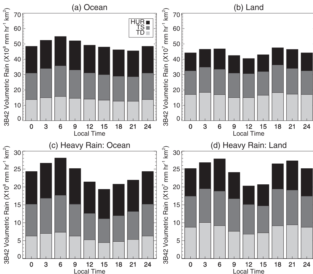
FIG. 13. Diurnal variations of volumetric rain for all 3B42 TCPFs over (a) ocean and (b) land, and for heavy rain regions only in 3B42 TCPFs over (c) ocean and (d) land from 1998 to 2009. Volumetric rains from different storm intensity categories (e.g., HUR, TS, and TD) are shown in different shades.
