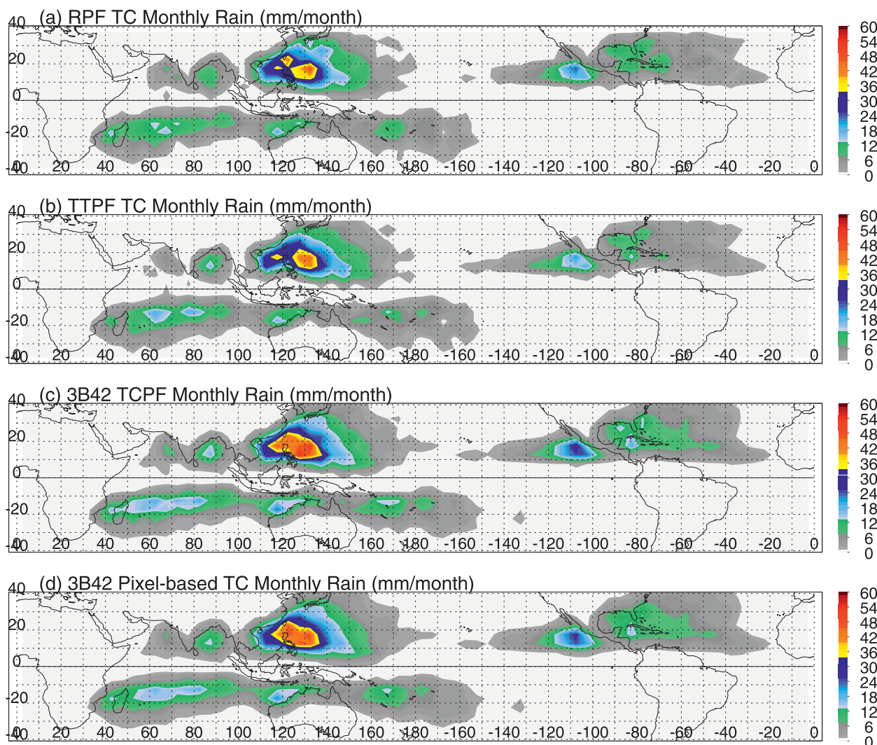
FIG. 7. (a) Mean 2A25 TC monthly rain from RPFs from 1998 to 2009. (b) Mean 2A12 TC monthly rain from TTPFs from 1998 to 2009. (c) Mean 3B42 TC monthly rain from 3B42 TCPFs from 1998 to 2009. (d) Mean 3B42 TC monthly rain from 3B42 TCPF level-1 raining pixels from 1998 to 2009.
