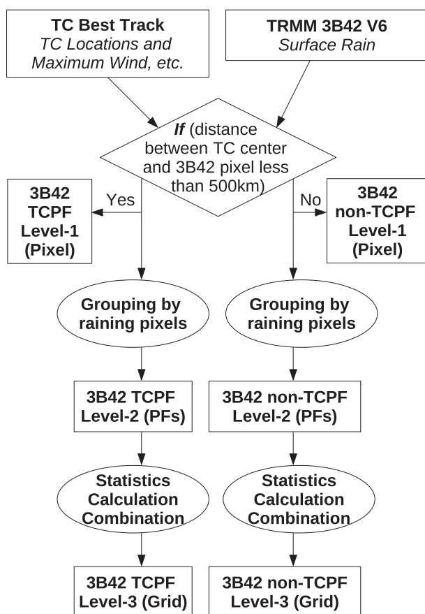
FIG. 5. FIU-UU TRMM 3B42 TCPF database construction flowchart.
