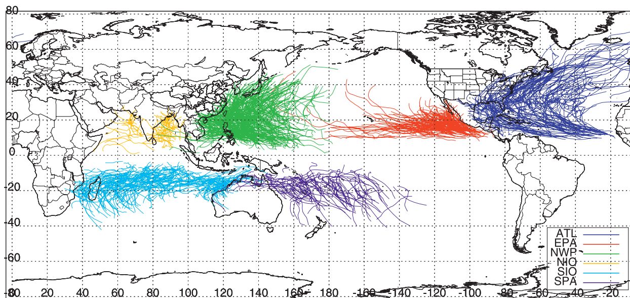
FIG. 2. Global TC best tracks in six basins during 1998–2009.
