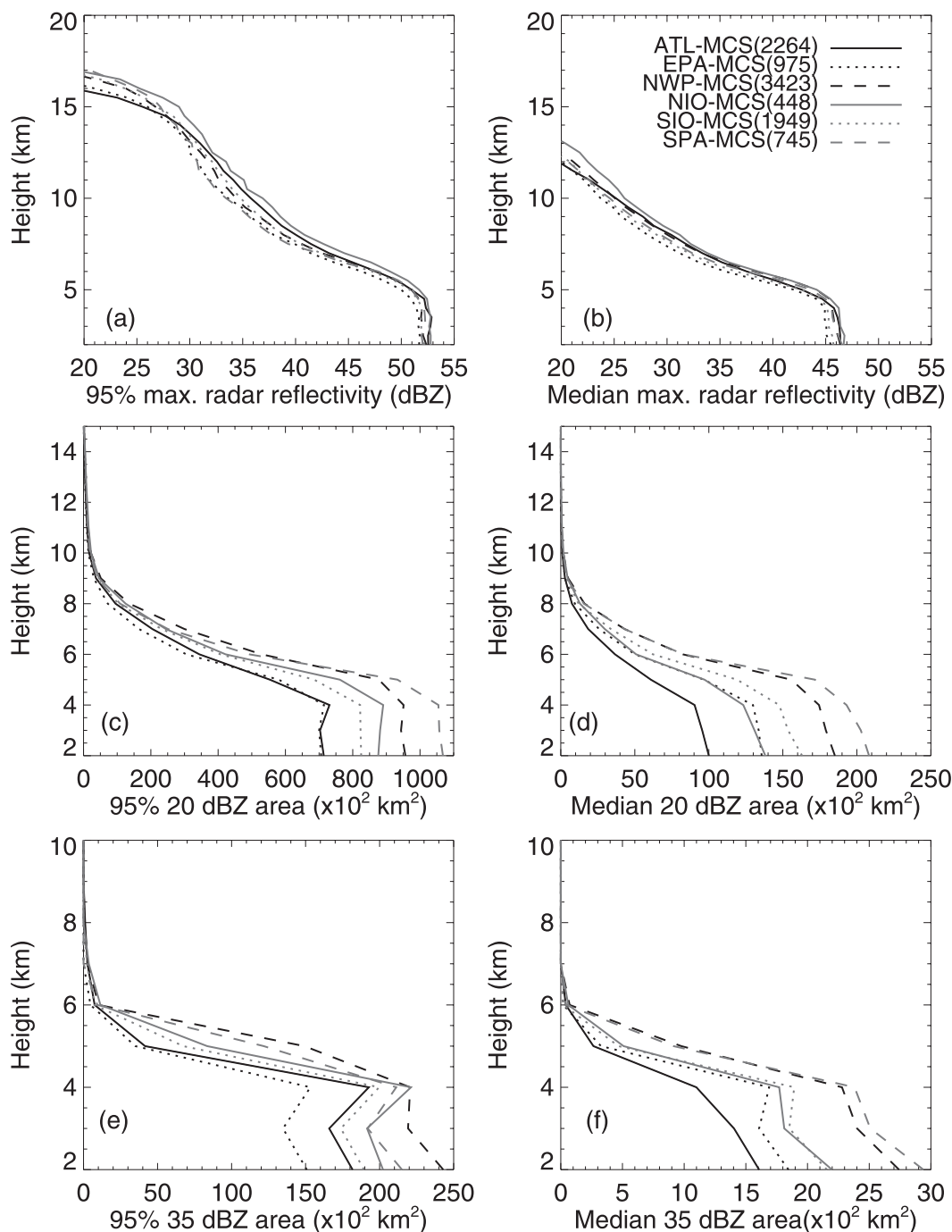
FIG. 11. The 95th percentile and median of vertical profiles of (a),(b) maximum radar reflectivity, (c),(d) 20-dBZ area, and (e),(f) 35-dBZ area of TC MCSs from 1998 to 2009 over six basins. Note that scales are different for (a)–(f).
