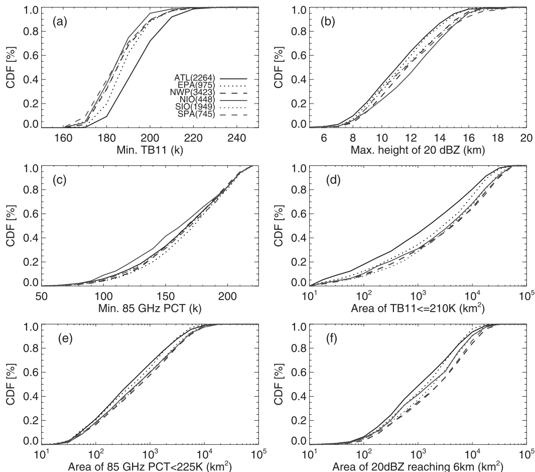
FIG. 9. Cumulative distribution functions (CDFs) of convective intensity inferred from (a) minimum T_{B11} , (b) maximum height of 20-dBZ echo, and (c) minimum 85-GHz PCT and CDFs of convective area inferred from (d) area of T_{B11} \leq 210 K, (e) area of minimum 85-GHz PCT < 225 K, and (f) area of 20 dBZ reaching 6 km over six basins for TC MCSs (derived from RPPFs; see text for details) from 1998 to 2009. TC MCS sample size of each basin is indicated.
