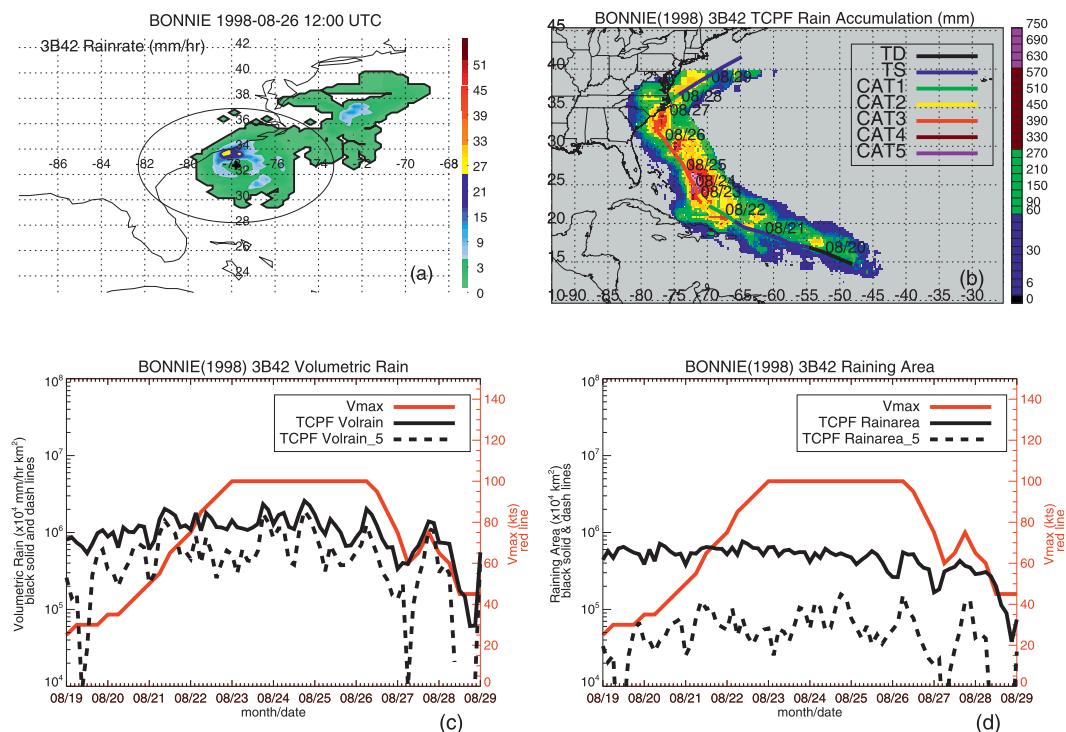
FIG. 6. Demonstration of 3B42 TCPF feature and parameters using the case of Hurricane Bonnie (1998). (a) 3B42 rain rate at 1200 UTC 26 Aug 1998. 3B42 TCPF feature is defined by the area both with rain rate >0 \text{ mm h}^{-1} (black contour) and within the 500-km radius circle around the hurricane center. (b) Lifetime total rain accumulation from 3B42. (c) Time series of 3B42 TCPF volumetric rain for all rain regions and heavy rain regions (rain rate > 5 \text{ mm h}^{-1} ). (d) Time series of 3B42 TCPF raining area for all rain regions and heavy rain regions (rain rate > 5 \text{ mm h}^{-1} ). The 500-km radius circle around the storm center is indicated in (a). Bonnie's best track is indicated in (b). The time series of Bonnie's maximum surface wind speed is indicated in (c) and (d).
