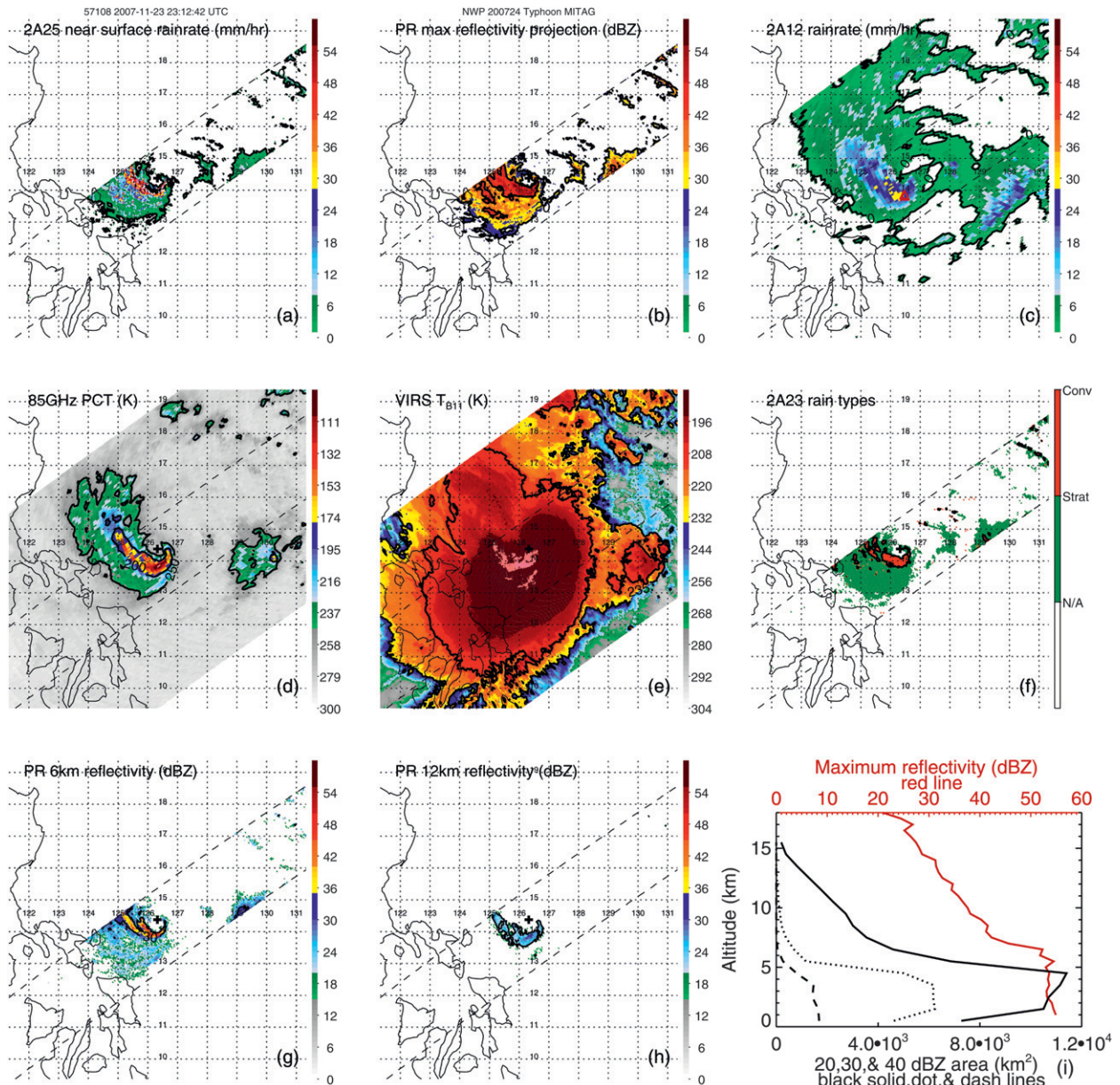
FIG. 4. Demonstration of the TCPF feature types using the case of Typhoon Mitag (2007). (a) 2A25 near-surface rain rate. RPF is defined by the area with rain shown by black contour. (b) The PR maximum-reflectivity ground projection. RPPF (CL40PF) is defined by area with 20 dBZ (40 dBZ) shown by black contours. (c) 2A12 surface rainfall rate. TTPF (TPF) is defined by area with rain shown by black contour in TMI (PR) swath. Red triangles are the location of flashes detected by LIS (note that there are two flashes in the same location; also see Table 2). (d) TMI 85-GHz PCT. TPCTF (T200F) is shown by 250-K (200 K) contour line. (e) VIRS T_{B11} C210F and C235F are defined by area with T_{B11} < 210 and 235 K shown by black contours inside the PR swath. (f) 2A23 rain types. CLCONVF is defined by area with spatially adjacent convective pixels shown by black contours. (g) The PR 6-km reflectivity. CL6KM30F is defined by the area with 30 dBZ at 6 km as shown by black contour. (h) The PR 12-km reflectivity. CL12KM20F is defined by the area with 20 dBZ at 12 km as shown by black contour. (i) Vertical profiles of 20-, 30-, and 40-dBZ area (black solid, dotted, and dashed lines, respectively) and the maximum reflectivity (red line) of the large RPPF defined in (b). The plus sign at the center of (a)–(h) is the typhoon center location. The dashed line in (a)–(h) is the edge of the PR swath. Note that there could be a truncation effect due to the narrow swath in defining large features (Nesbitt et al. 2006).
