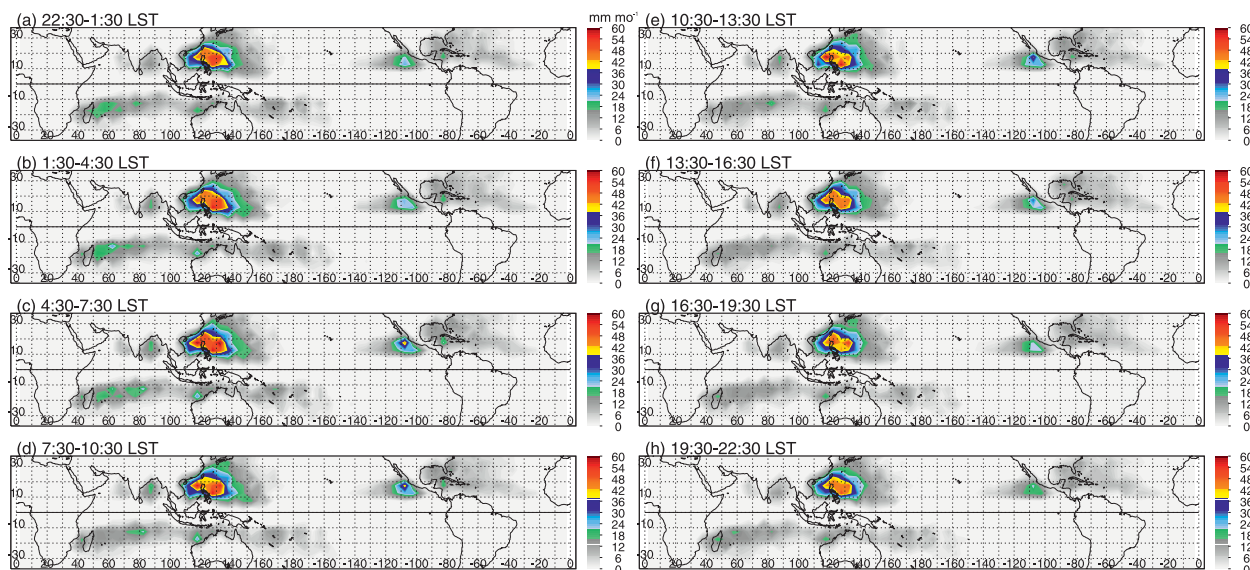
FIG. 12. The 3B42 TC monthly rain from 1998 to 2009 at (a) 2230–0130, (b) 0130–0430, (c) 0430–0730, (d) 0730–1030, (e) 1030–1330, (f) 1330–1630, (g) 1630–1930, and (h) 1930–2230 LST.
